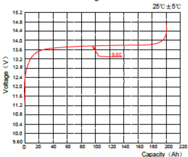
charge curve
